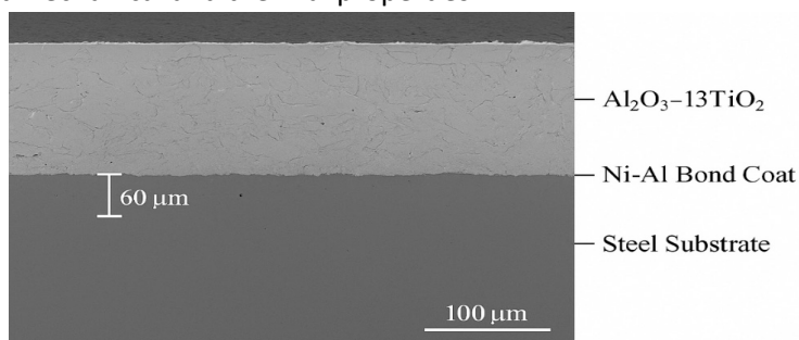
Figure 5. SEM micrograph of the cross-section of the \text{Al}_2\text{O}_3 -13TiO 2 coating on the steel substrate, which indicates the bond coat as well as structure of the lamellar topcoat.
